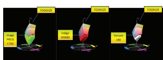
Figure 2. 3D visualisation (Lab system) of an ICC profile of offset paper printed through CANON imagePRESS C750, HP Indigo WS 6800 and Xerox Versant 180 Press and FOGRA29
