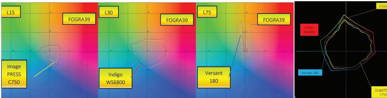
Figure 12. Graphic representation and comparison of 2D colour gamut with different values of L over coated paper, as printed by CANON imagePRESS C750, HP Indigo WS 6800 and Xerox Versant 180 Press compared with reference values as per FOGRA39
