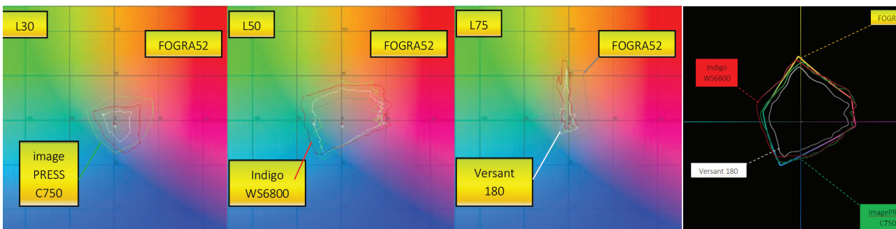
Figure 11. Graphic representation and comparison of 2D colour gamut with different values of L over uncoated paper, as printed by CANON imagePRESS C750, HP Indigo WS 6800 and Xerox Versant 180 Press compared with reference values as per FOGRA52
