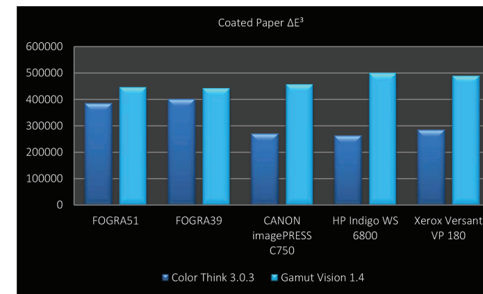
Figure 15 Graphic representation of the colour gamut \Delta E3 for Coated Paper as printed by CANON imagePRESS C750, HP Indigo WS 6800 and Xerox Versant 180 compared with reference values as per FOGRA calculated with CHROMIX Color Think 3.0.3 and Gamut Vision 1.4
