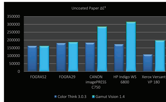
Figure 14 Graphic representation of the colour gamut \Delta E3 for Uncoated Paper as printed by CANON imagePRESS C750, HP Indigo WS 6800 and Xerox Versant 180 compared with reference values as per FOGRA calculated with CHROMIX Color Think 3.0.3 and Gamut Vision 1.4
