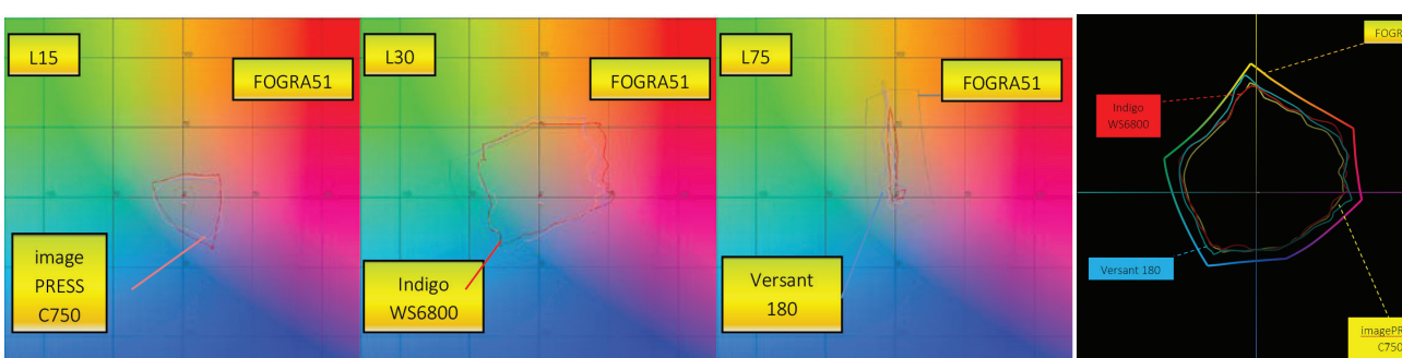
Figure 13. Graphic representation and comparison of 2D colour gamut with different values of L over coated paper, as printed by CANON imagePRESS C750, HP Indigo WS 6800 and Xerox Versant 180 Press compared with reference values as per FOGRA51
